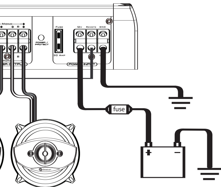
Connection Diagram: Front of Full Range Speakers (80Hz Highpass)
